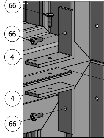
DETAIL A-1
