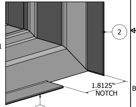
DETAIL C-1
